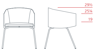
Armchair on four legs 1PL6030: L 25½ D 23 H 29½
