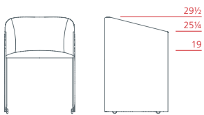
Tall armchair on castors 1PL6011: L 22 D 20 H 29½
