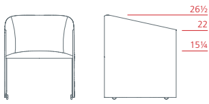
Lounge armchair on castors 1PL6021: L 22 D 22¾ H 26½
